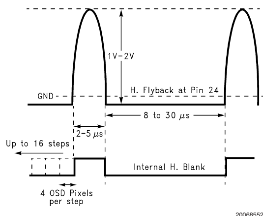
FIGURE 12. Programmable Internal H. Blank
