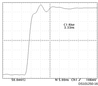
FIGURE 7. LM1279A Rise Time
