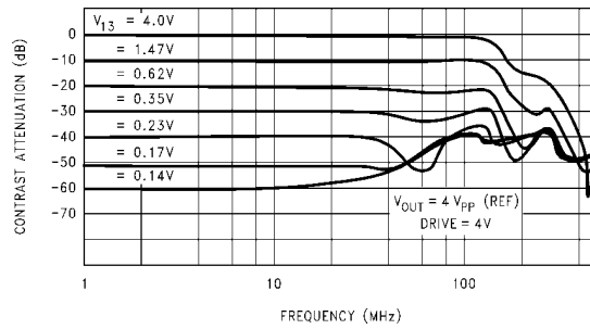
LM1282 Contrast vs Frequency
