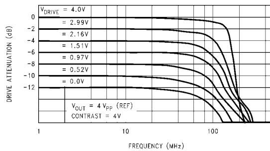
LM1282 Drive vs Frequency
