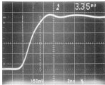
FIGURE 8a. LM1282 Rise Time
