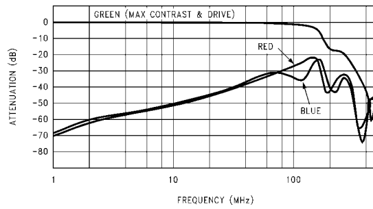
LM1282 Crosstalk vs Frequency
