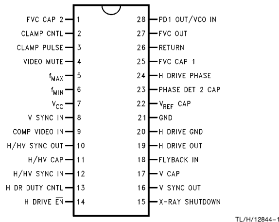
FIGURE 1 Order Number LM1292N See NS Package Number N28B
