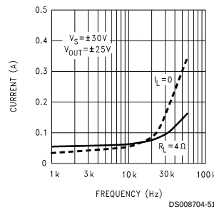
Cross-Supply Current
