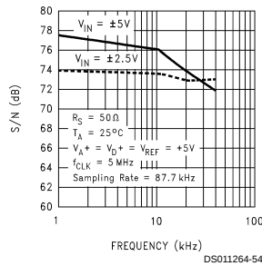
Bipolar Signal-to-Noise Ratio vs Input Frequency
