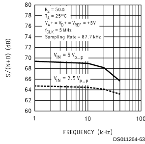
Unipolar Signal-to-Noise + Distortion Ratio vs Input Frequency
