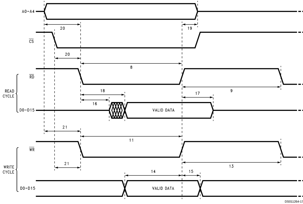
FIGURE 11. Non-Multiplexed Data Bus (ALE = 1)
