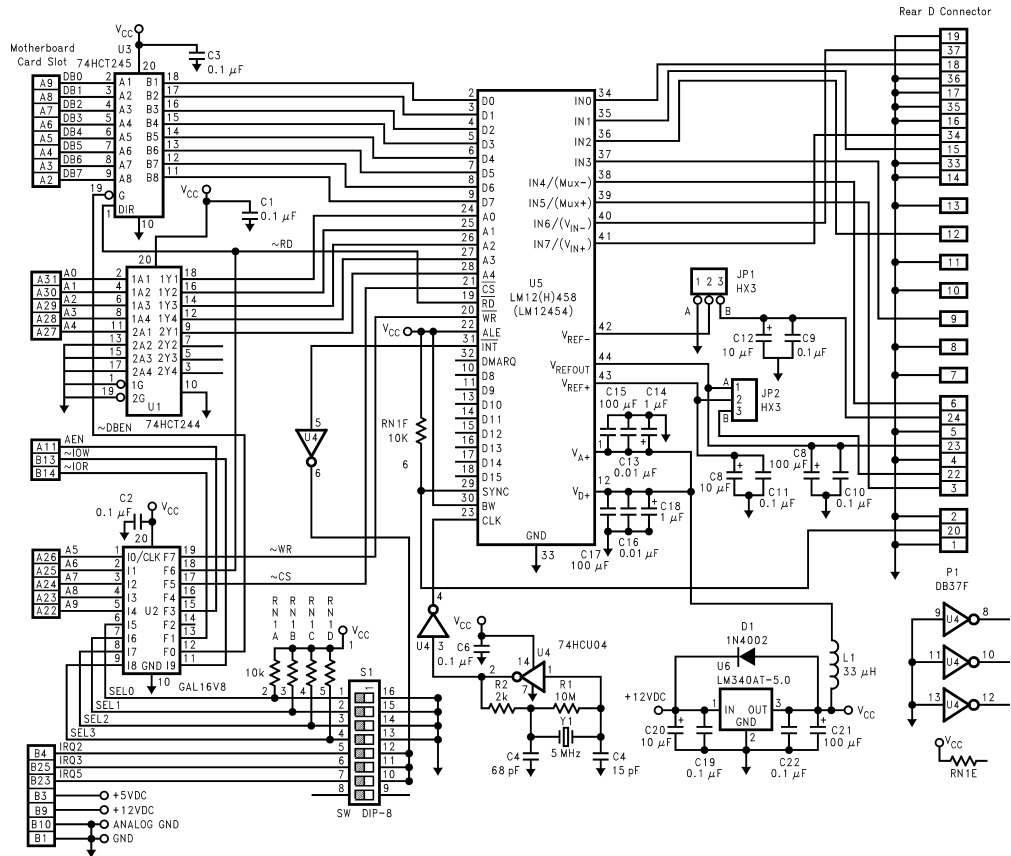
FIGURE 16. Schematic for the LM12(H)454/8 Evaluation Interface Board for XT and AT Style Computers, Order Number LM12458EVAL
