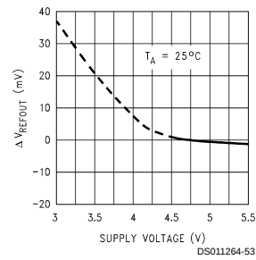
V REFOUT Line Regulation
