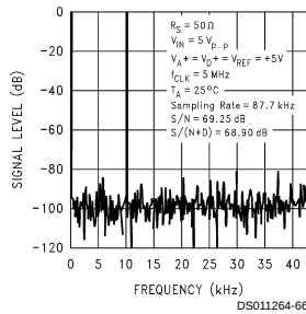
Unipolar Spectral Response with 10 kHz Sine Wave Input
