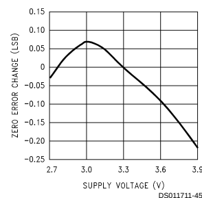
Zero Error Change vs Supply Voltage
