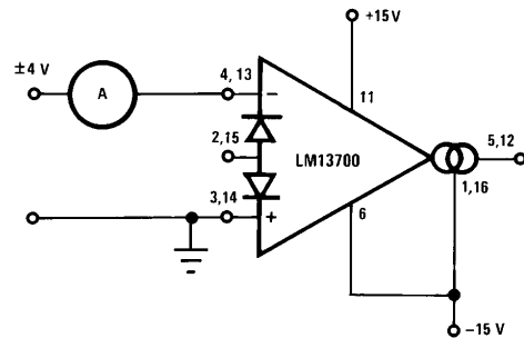
Differential Input Current Test Circuit
