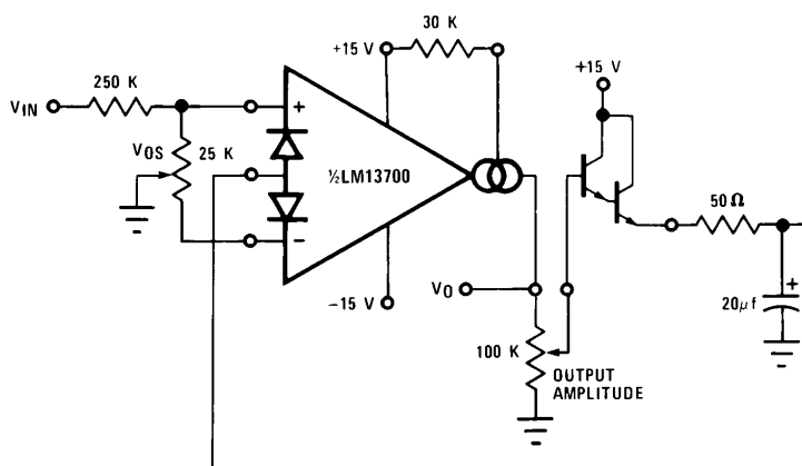
FIGURE 7. AGC Amplifier
