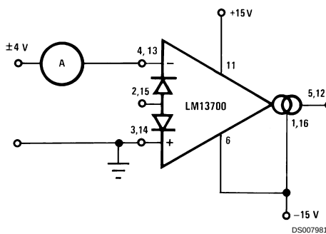
Differential Input Current Test Circuit
