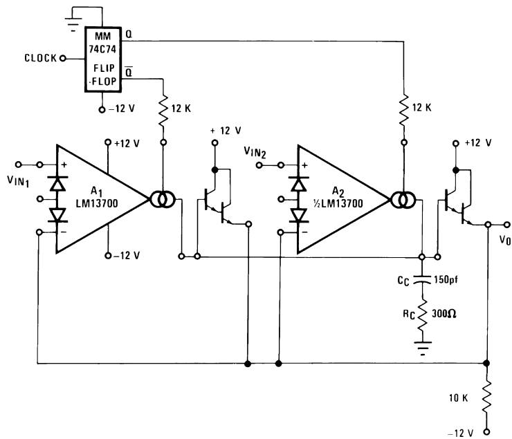
FIGURE 20. Multiplexer
