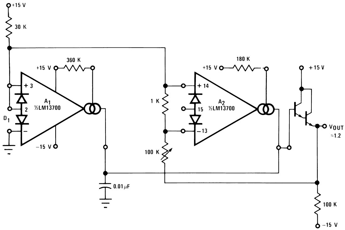
FIGURE 28. Delta VBE Reference
