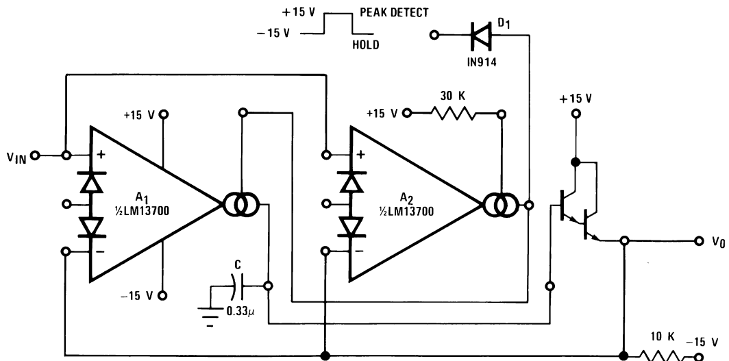
FIGURE 24. Peak Detector and Hold Circuit
