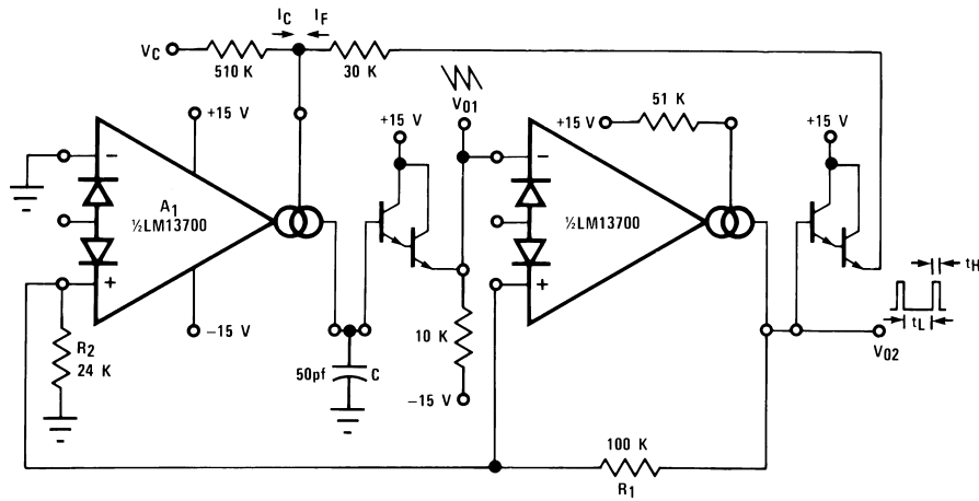
FIGURE 15. Triangular/Square-Wave VCO
