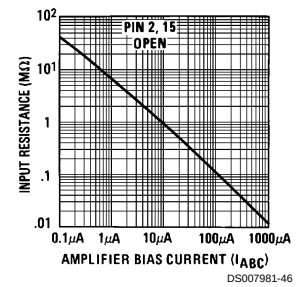
Input Resistance
