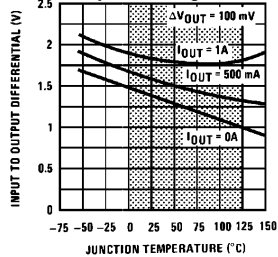
Dropout Voltage
