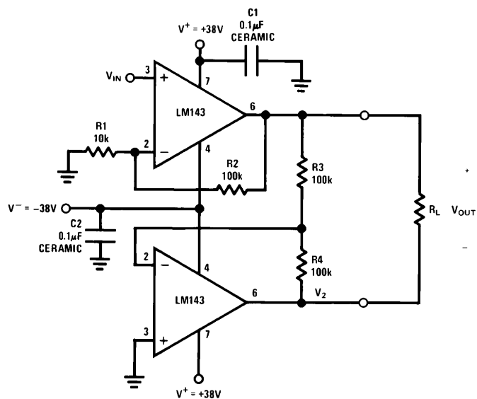
130 V p-p Drive Across a Floating Load
