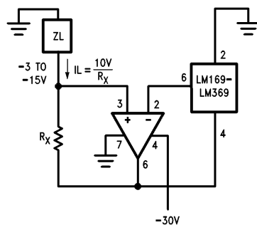
Current Source
