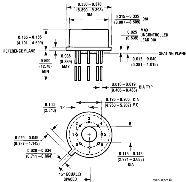
Metal Can Package (H) Order Number LM169BH, LM169H, LM169H/883, LM369BH or LM369H NS Package Number H08C
