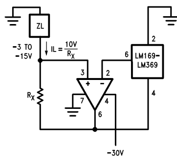
Current Source
