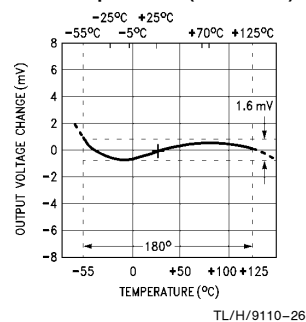
LM169 Temperature Coefficient Specified Temperatures (see Note 6)
