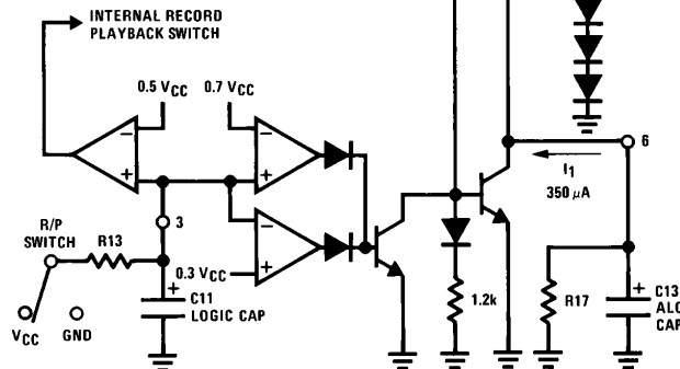
FIGURE 8A. Anti-Pop Circuit
