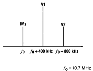
FIGURE 13. Spectrum Analyzer Display of Tuner Output
