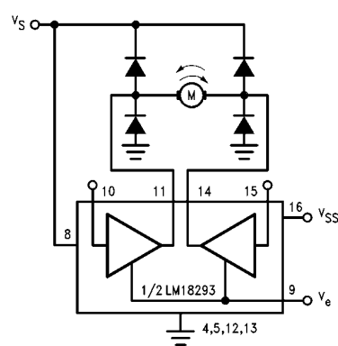
Bidirectional DC motor control
