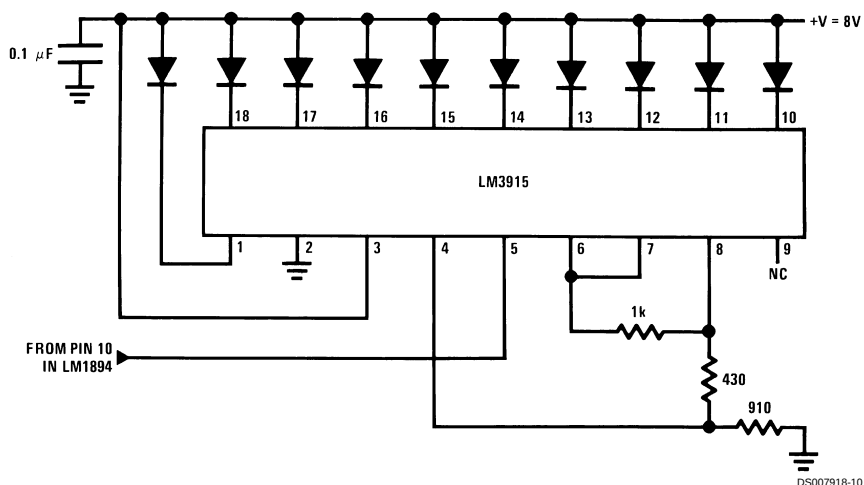
FIGURE 5. Bar Graph Display of Peak Detector Voltage
