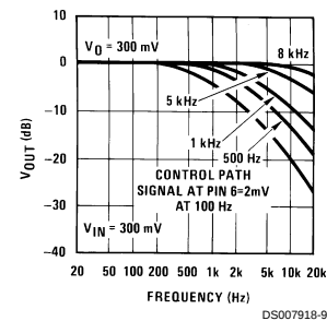
FIGURE 4. -3 dB Bandwidth vs Frequency and Control Signal
