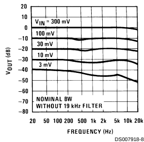
FIGURE 3. Output vs Frequency
