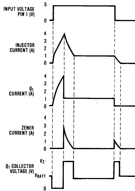
FIGURE 4. Circuit Waveforms
