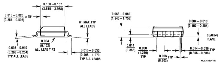
14-Lead (0.150" Wide) Molded Small Outline Package, JEDEC Order Number LM1949M NS Package Number M08A
