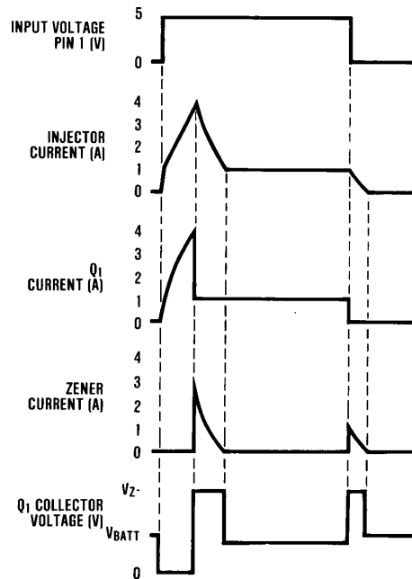
FIGURE 4. Circuit Waveforms
