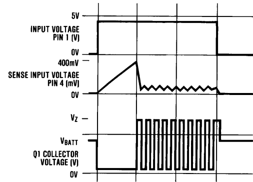
FIGURE 6. Switching Waveforms
