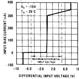
Input Characteristics
