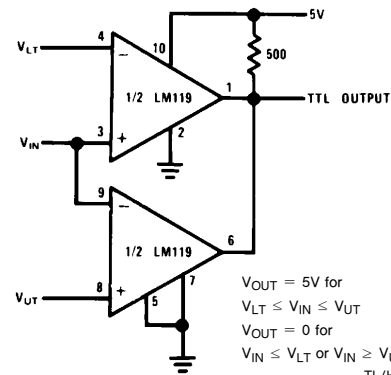
Window Detector
