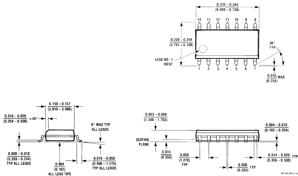
Dual-In-Line Package (M) Order Number LM319AM or LM319M NS Package Number M14A
