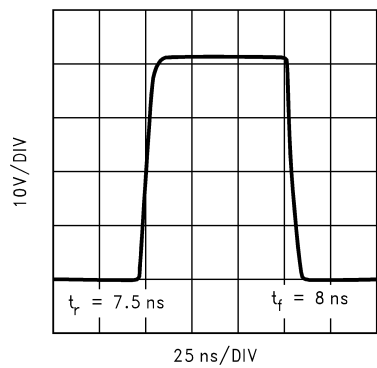
FIGURE 5. LM2466 Pulse Response
