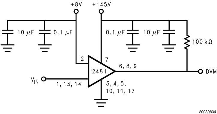
FIGURE 2. Test Circuit
