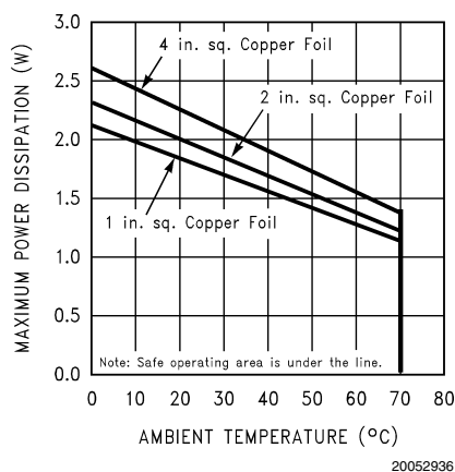
FIGURE 4. Maximum Power Dissipation vs. Ambient Temperature
