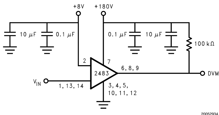
FIGURE 2. Test Circuit
