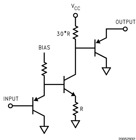
FIGURE 1. Simplified Schematic Diagram (One Channel)
