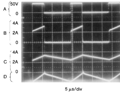
Switching Waveforms
