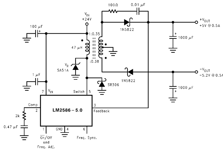
FIGURE 43. Flyback Regulator
