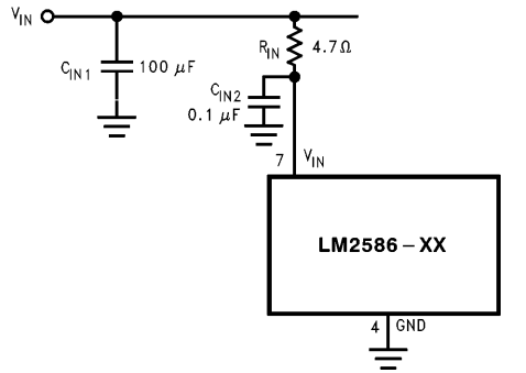
FIGURE 44. Input Line Filter
