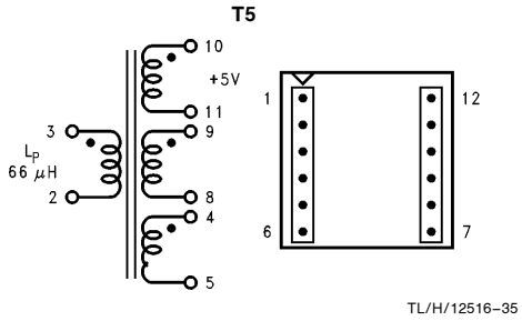
FIGURE 17. Coilcraft Q4437-B (Surface Mount)
