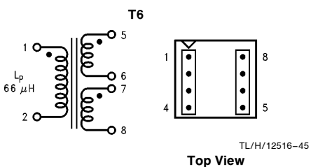
FIGURE 25. Renco RL-5533
