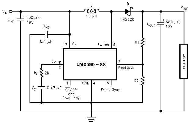
FIGURE 2. LM2586-12 and LM2586-ADJ
