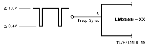
FIGURE 40. Frequency Synchronization
