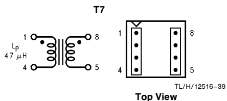
FIGURE 21. Pulse PE-68482
