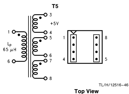
FIGURE 26. Renco RL-5532
