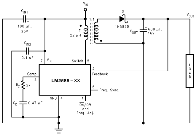
FIGURE 1. LM2586-3.3 and LM2586-5.0
