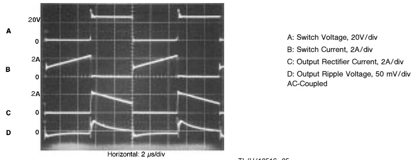
FIGURE 5. Switching Waveforms
