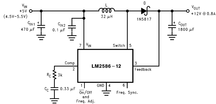
FIGURE 30. 12V Boost Regulator
