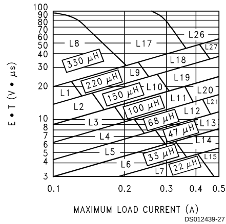
FIGURE 7. LM2594/LM2594HV-ADJ
