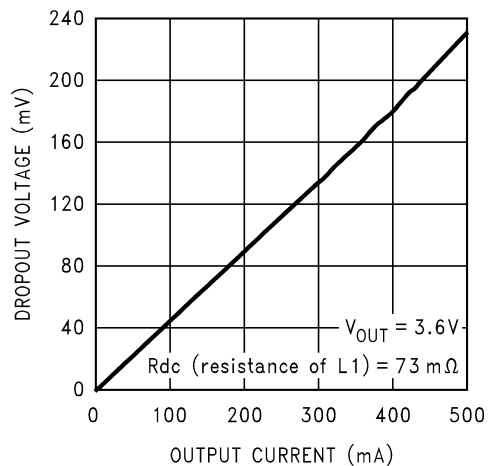
Dropout Voltage vs Output Current ( V_{OUT} = 3.6V , PWM MODE) (Circuit in Figure 4)
