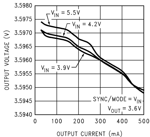
Output Voltage vs Output Current ( V_{OUT} = 3.6V , PWM MODE) (Circuit in Figure 4)
