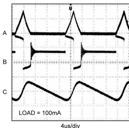
PFM Mode Switching Waveform
