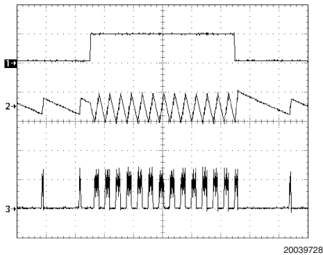
Step Response
