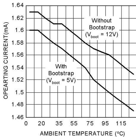
V_{CC} Operating Current vs Temperature F_{SW} = 600kHz , No-Load
