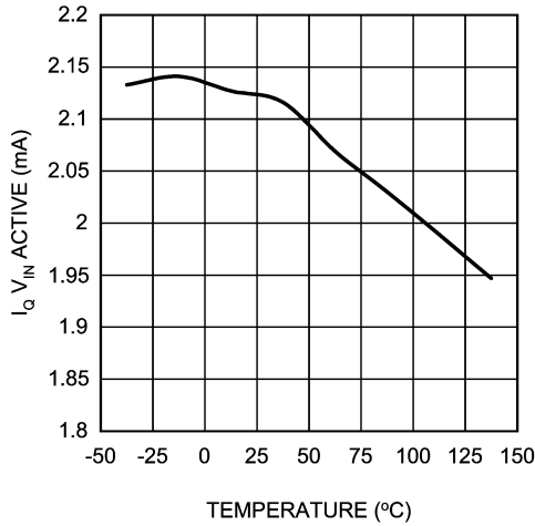
I Q Vin (Active) vs Temperature - "X"
