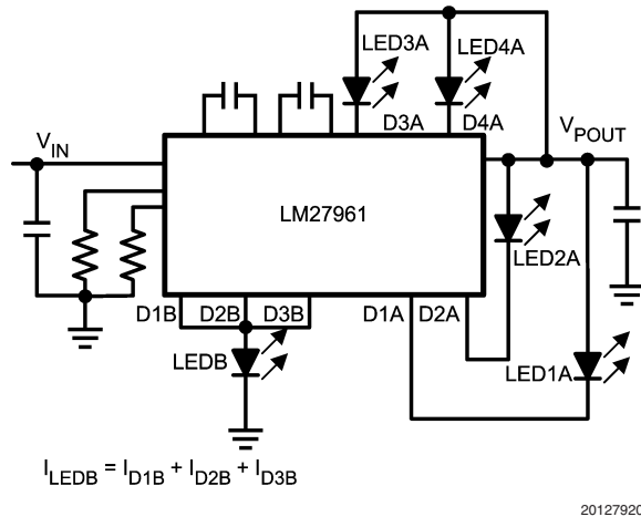
FIGURE 2. One Parallel Connected LED
