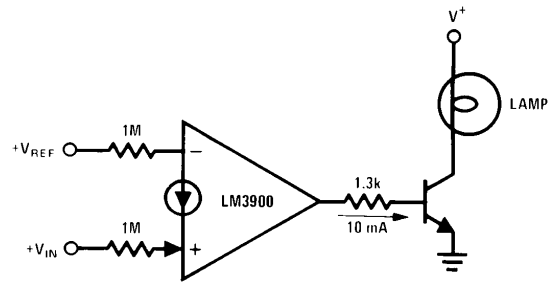
Power Comparator
