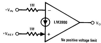
Comparator
