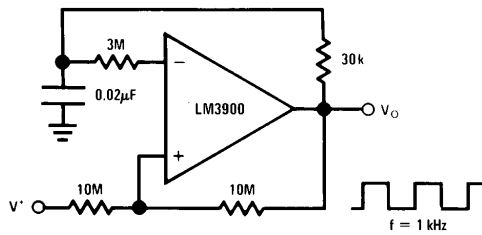
Square-Wave Oscillator
