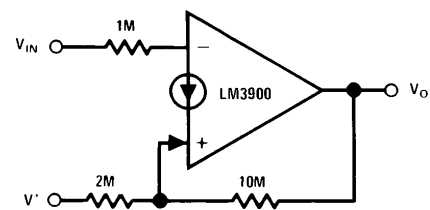
Schmitt-Trigger
