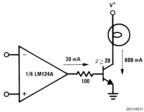
Lamp Driver
