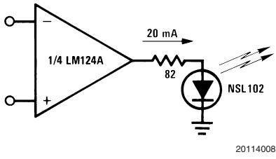
LED Driver
