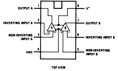
Dual-In-Line/SOIC Package
