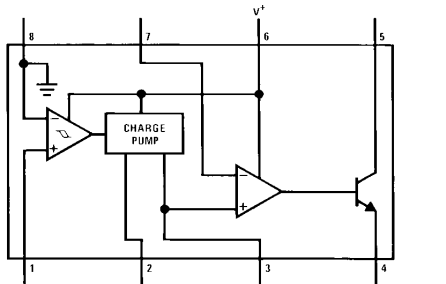
Order Number LM2907M-8 or LM2907N-8 See NS Package Number M08A or N08E
