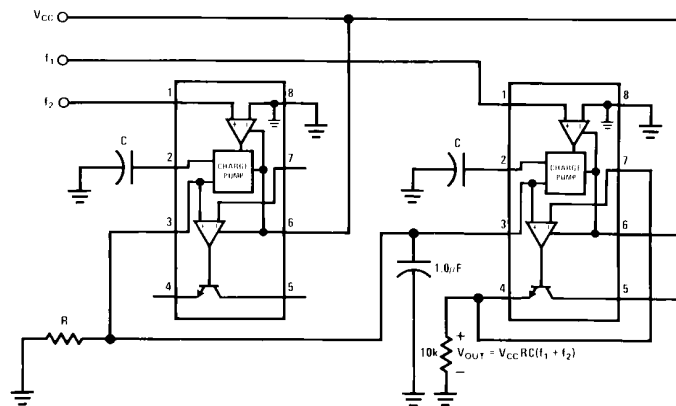
“Select-Average” Circuit
