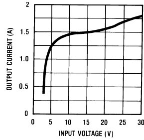
Peak Output Current ( V_{OUT} )
