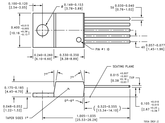
5-Lead TO-220 Power Package (T) Order Number LM2935T NS Package Number T05A
