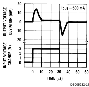
Line Transient Response ( V_{OUT} )
