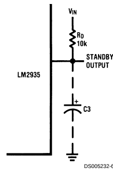
FIGURE 3. Disabling Standby Output to Eliminate C3
