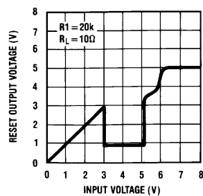
Reset on Startup
