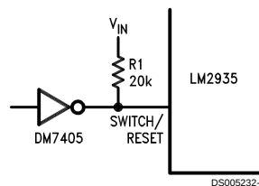
FIGURE 4. Controlling ON/OFF Terminal with a Typical Open Collector Logic Gate
