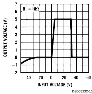
Output Voltage ( V_{OUT} )
