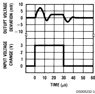
Line Transient Response ( V_{STBY} )
