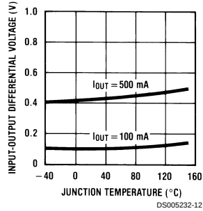
Dropout Voltage ( V_{OUT} )
