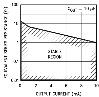
Output Capacitor ESR (Standby Output, Pin 5)
