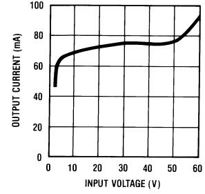
Peak Output Current ( V_{STBY} )
