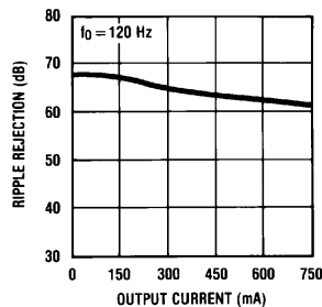
Ripple Rejection ( V_{OUT} )
