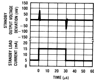
Load Transient Response ( V_{STBY} )
