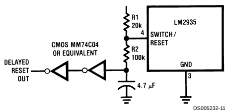
FIGURE 5. Reset Pulse on Power-Up (with approximately 300 ms delay)
