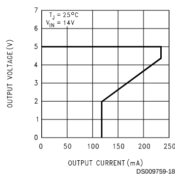
Current Limit
