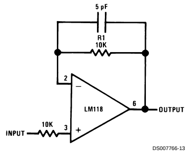
Fast Voltage Follower (Note 12)
