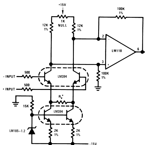
Instrumentation Amplifier
