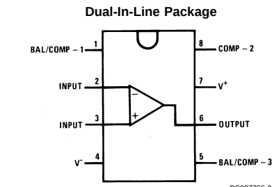
Top View Order Number LM118J-8/883 (Note 2), LM318M or LM318N See NS Package Number J08A, M08A or N08B
