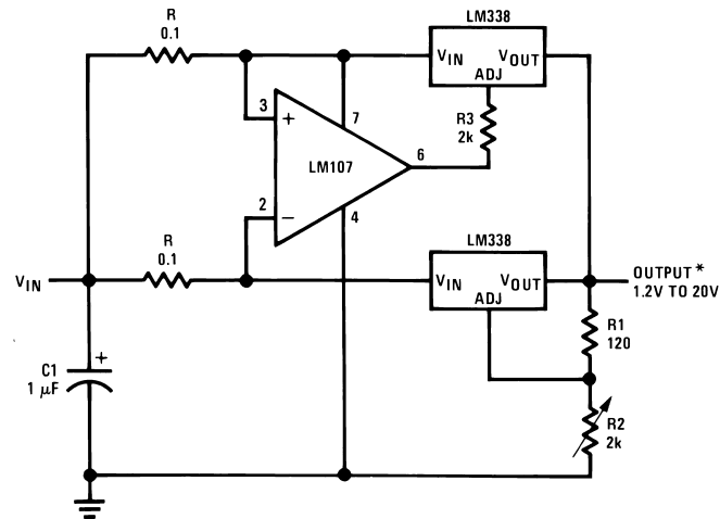
10A Regulator
