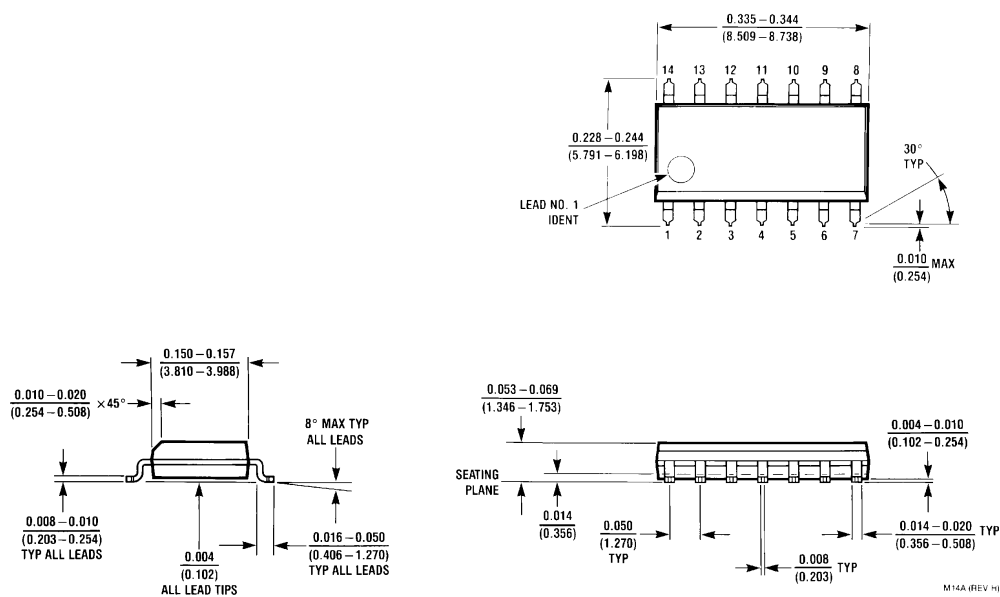
S.O. Package (M) Order Number LM339AM, LM339M or LM2901M NS Package Number M14A
