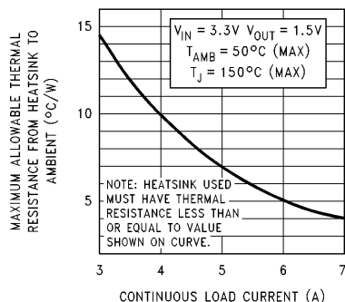
FIGURE 6. Q4 Heatsink Requirements for Circuit Shown in Figure 1
