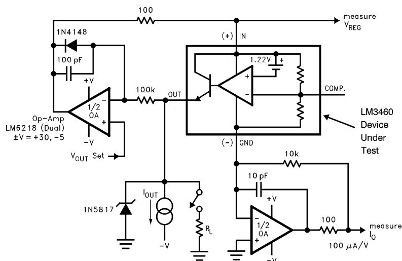
FIGURE 3. Test Circuit
