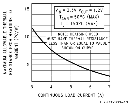
FIGURE 7. Q4 Heatsink Requirements for Circuit Shown in Figure 2
