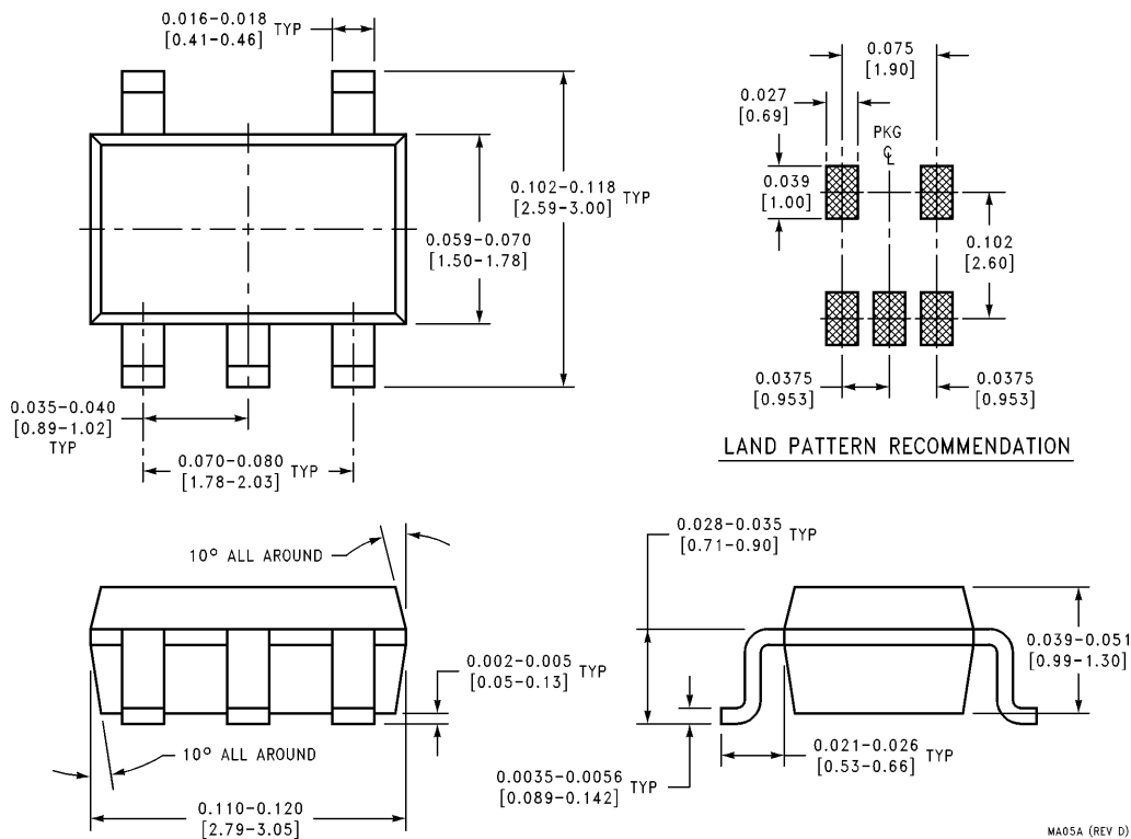
5-Lead Small Outline Package (M5) Ordering Number, See Page 1 of this Document NS Package Number MA05A
