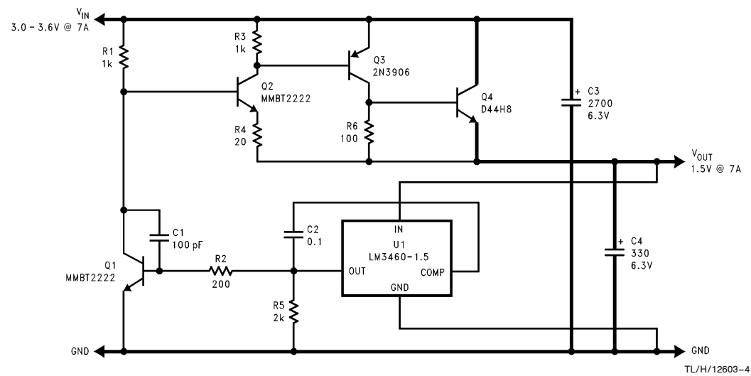
FIGURE 1. 1.5V Typical Application (See Application Information Section)
