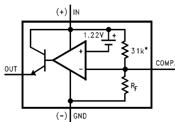
LM3460 Functional Diagram
