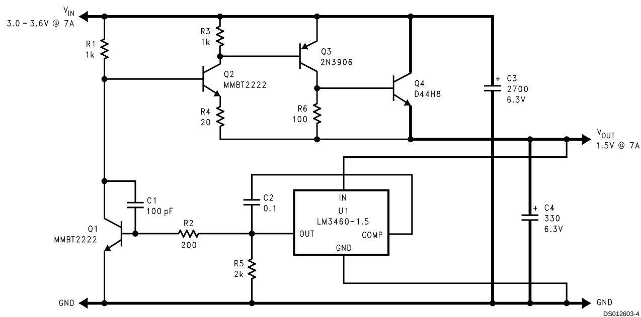
FIGURE 1. 1.5V Typical Application (See Application Information Section)
