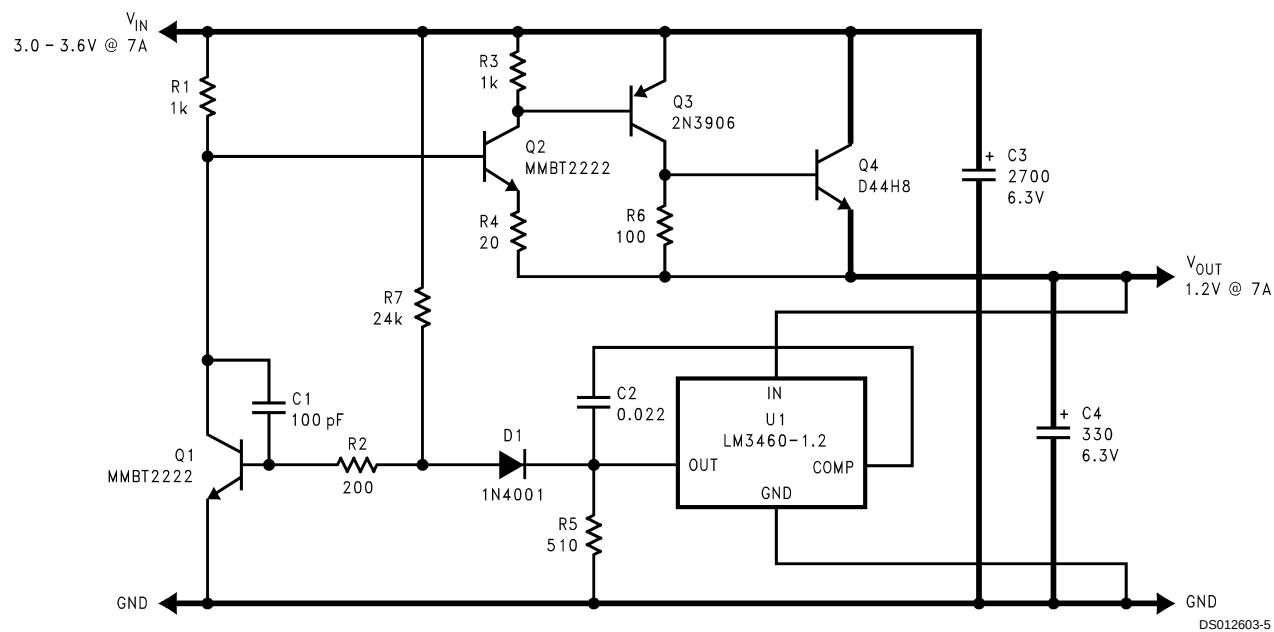
FIGURE 2. 1.2V Typical Application (See Application Information Section)
