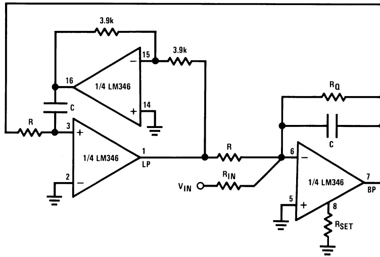
A Simple-to-Design BP, LP Filter Building Block
