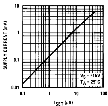
Supply Current vs I_{SET}
