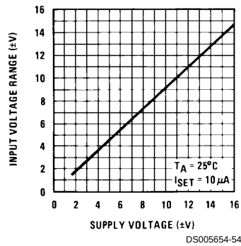
Input Voltage Range vs Supply Voltage
