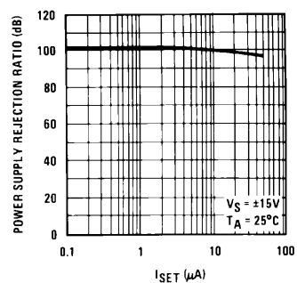
Power Supply Rejection Ratio vs I_{SET}
