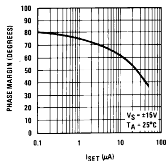
Phase Margin vs I_{SET}
