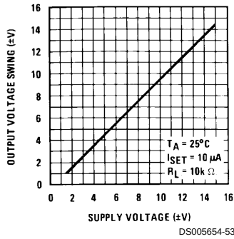
Open Voltage Swing vs Supply Voltage
