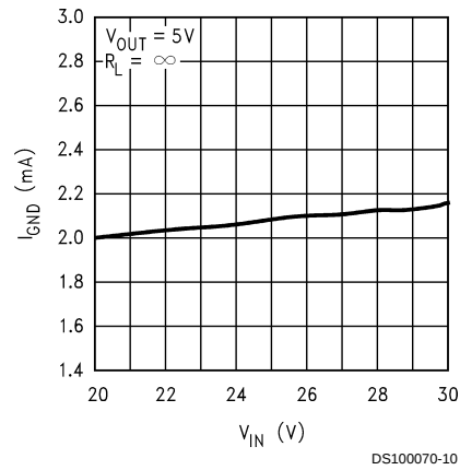
Ground Pin Current vs Input Voltage
