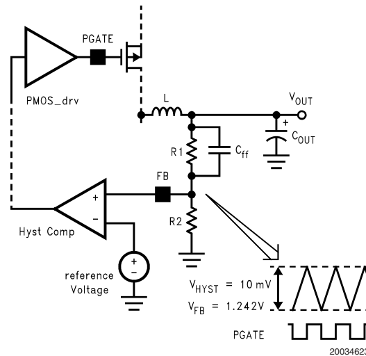
FIGURE 1. Hysteretic Window
