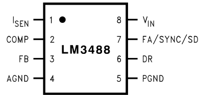
8 Lead Mini SO8 Package (MSOP-8 Package)
