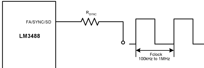
FIGURE 7. Frequency Synchronization
