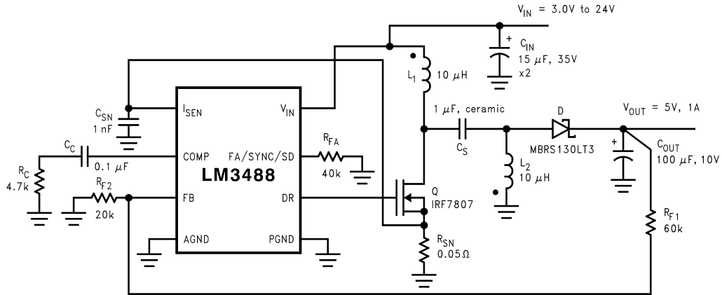
FIGURE 14. Typical SEPIC Converter
