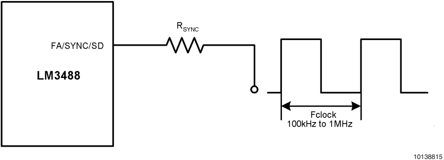
FIGURE 7. Frequency Synchronization
