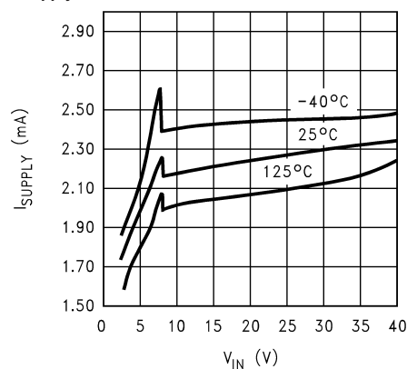
I_{SUPPLY} vs Input Voltage (Non-Switching)
