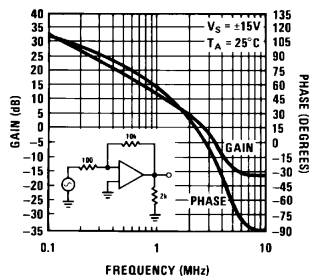
Bode Plot LM149
