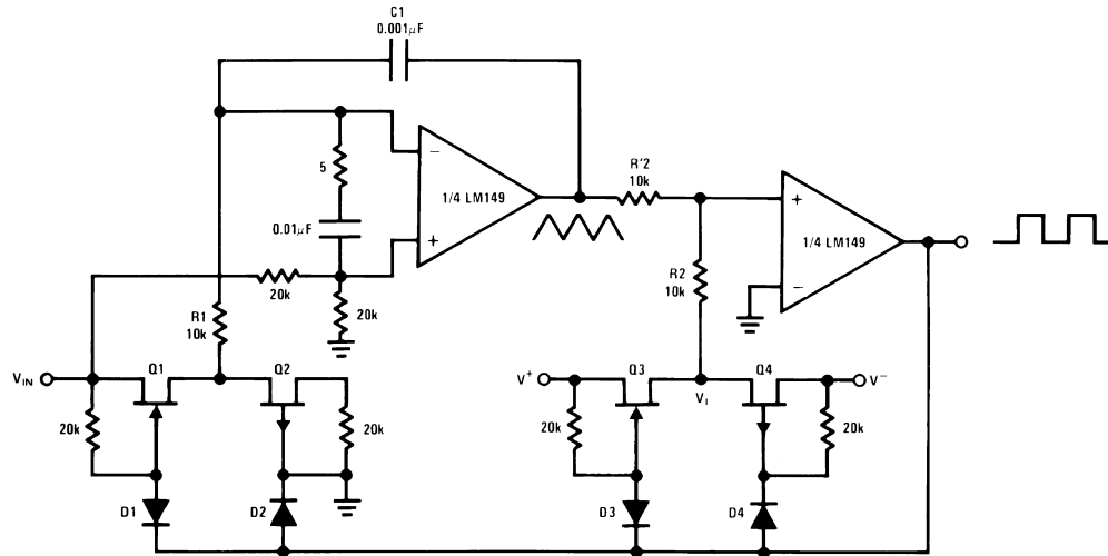
Triangular Squarewave Generator
